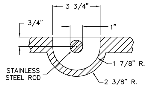
(2) TYPE 4 STEEL PICKBARS PICKBAR DETAIL
