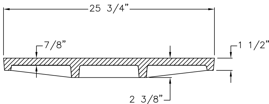
COVER SECTION
