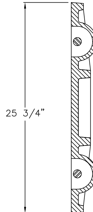
COVER SECTION
